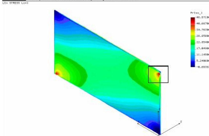
Fig. 8.4.6: Principle tensile stress P1 in [MPa], outboard lite
