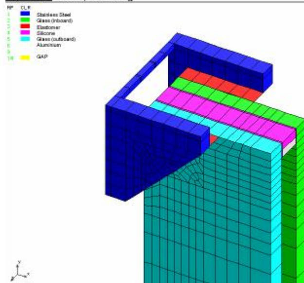
Fig. 8.2.2: Detail point fixing
